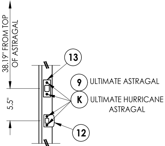
LATCH AND DEADBOLT STRIKE DETAILS
