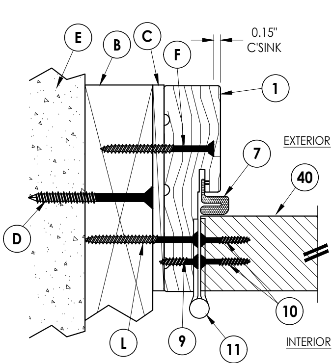
1 4 HORIZONTAL CROSS SECTION Inswing shown (Outswing similar) 2X Buck Construction
