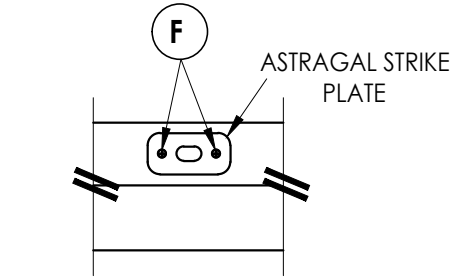
ASTRAGAL BOLT DETAIL Strike Plate @ Head
