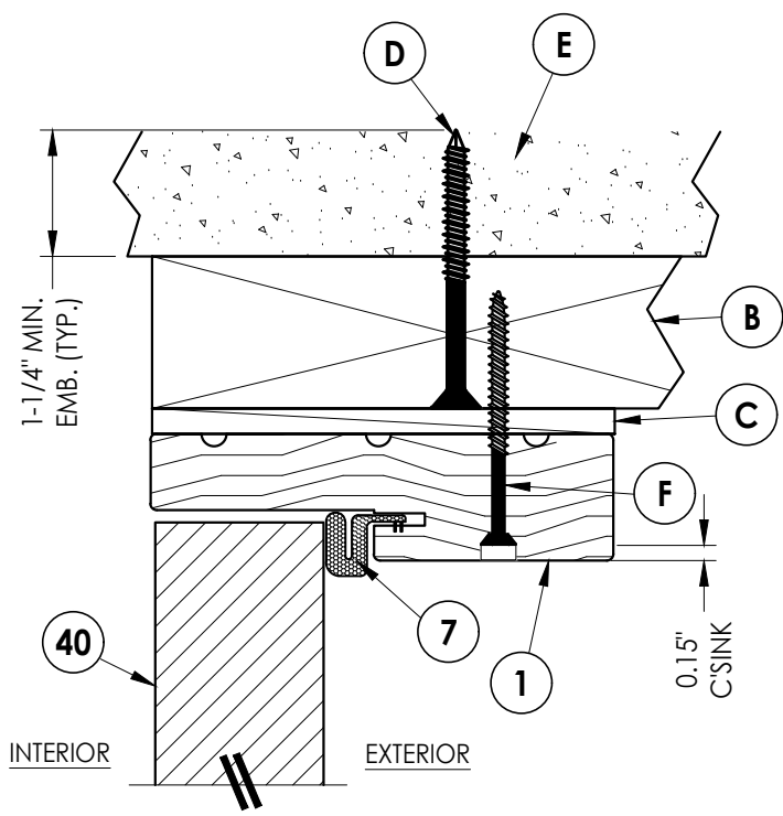
3 4 VERTICAL CROSS SECTION Inswing shown (Outswing similar) 2X Buck Construction
