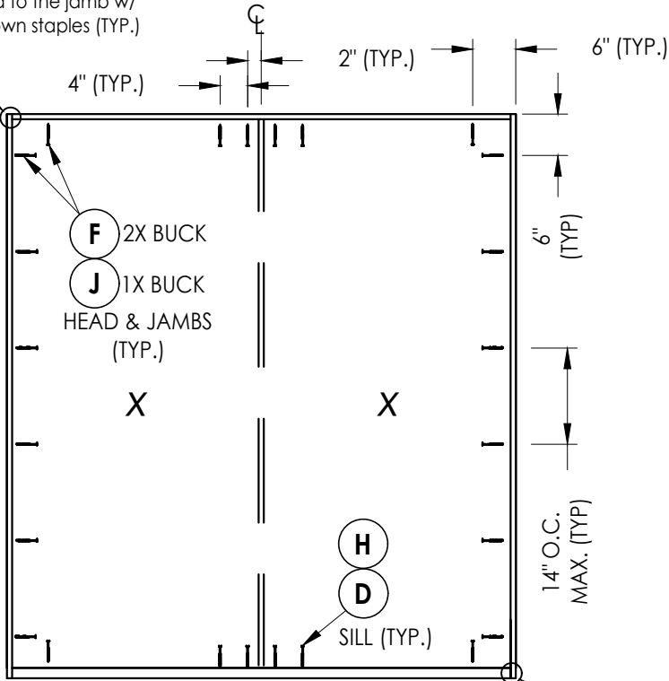
FRAME ANCHORING
