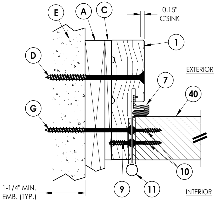
2 4 HORIZONTAL CROSS SECTION Inswing shown (Outswing similar) 1X Buck Construction
