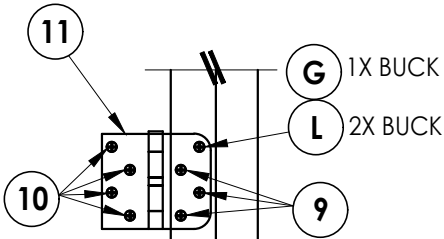
HINGE DETAIL 1
