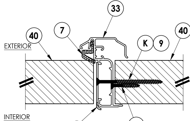
4 4 VERTICAL CROSS SECTION Inswing shown (Outswing similar) 1X Buck Construction
