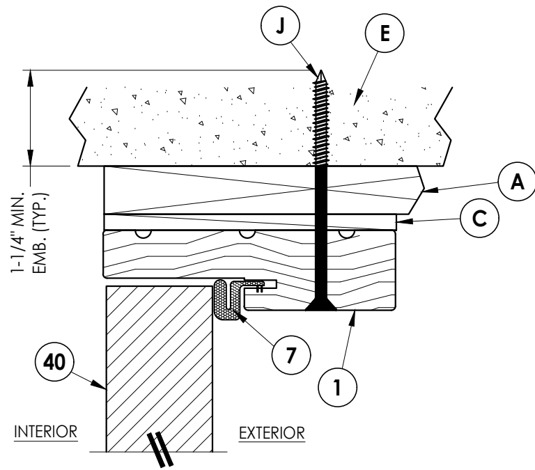
4 4 VERTICAL CROSS SECTION Inswing shown (Outswing similar) 1X Buck Construction
