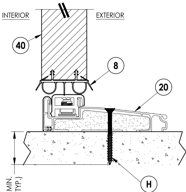
6 4 VERTICAL CROSS SECTION Inswing sill
