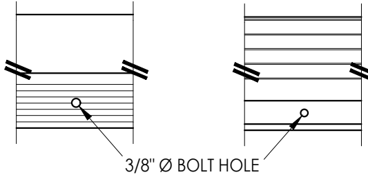
ASTRAGAL BOLT DETAIL Outswing Threshold
