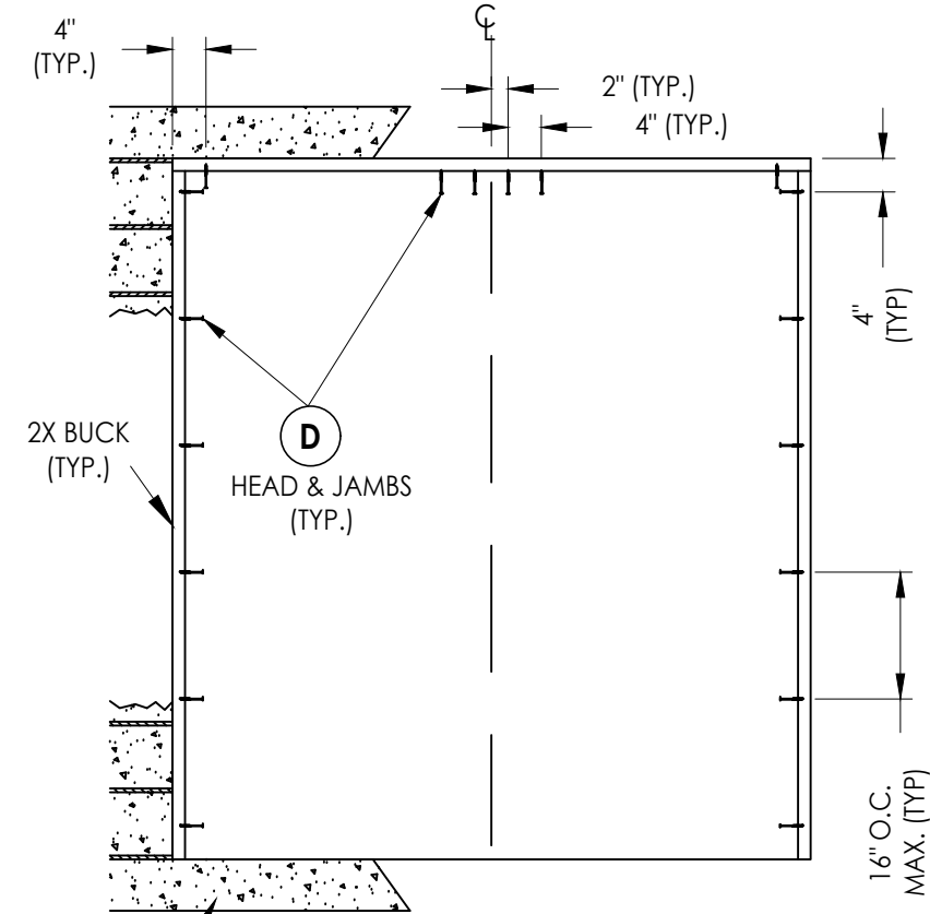
2X BUCK ANCHORING
