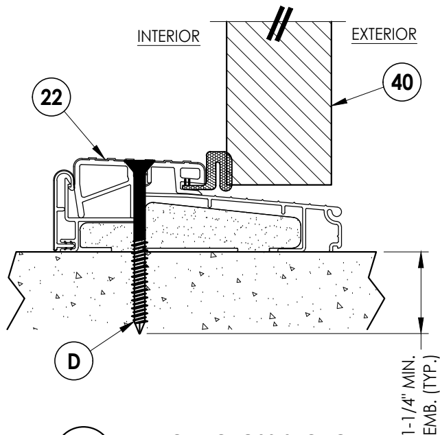
7 4 VERTICAL CROSS SECTION Outswing sill
